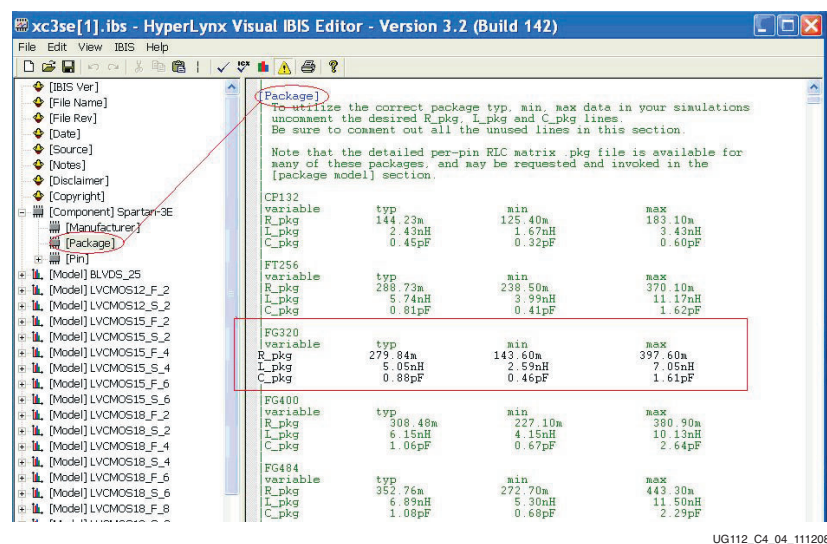
Figure 4-4: Embedded Electrical Parasitics Data
