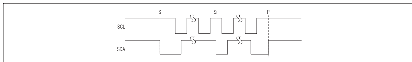
Figure 33. START, STOP, and REPEATED START Conditions
