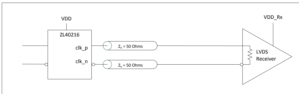
Figure 13 - LVDS DC Coupled Termination (Internal Receiver Termination)
