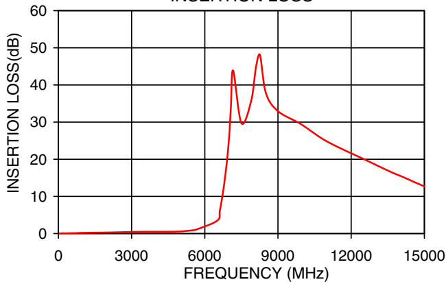
LFCN-5850D+ INSERTION LOSS
