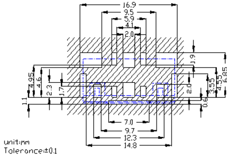
3-2-2 Solder resist Patten
