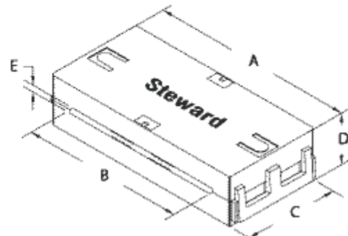
Figure #4 Split ferrite core assembly with hinged black plastic case
