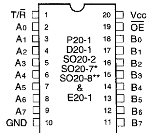
DIP/SOIC/SSOP/QSOP/CERPACK TOP VIEW
