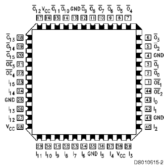
Pin Assignment for PCC
