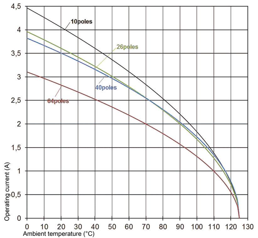
Derating curve 80%
