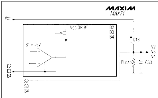
Figure 2. Functional Diagram and Circuit for Linear Regulators V2-V4
