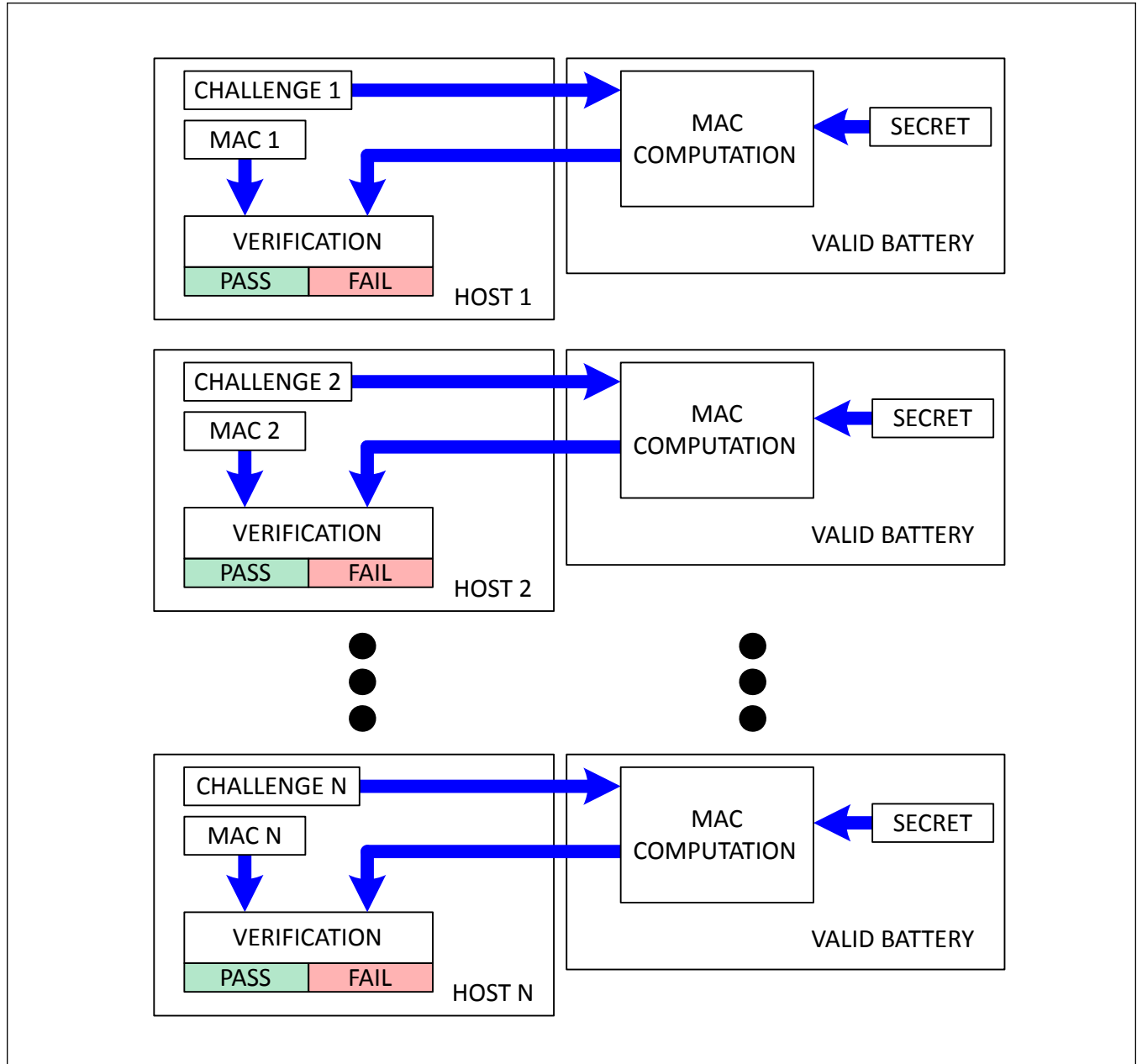
Figure 27. Battery Authentication without a Host Side Secret
