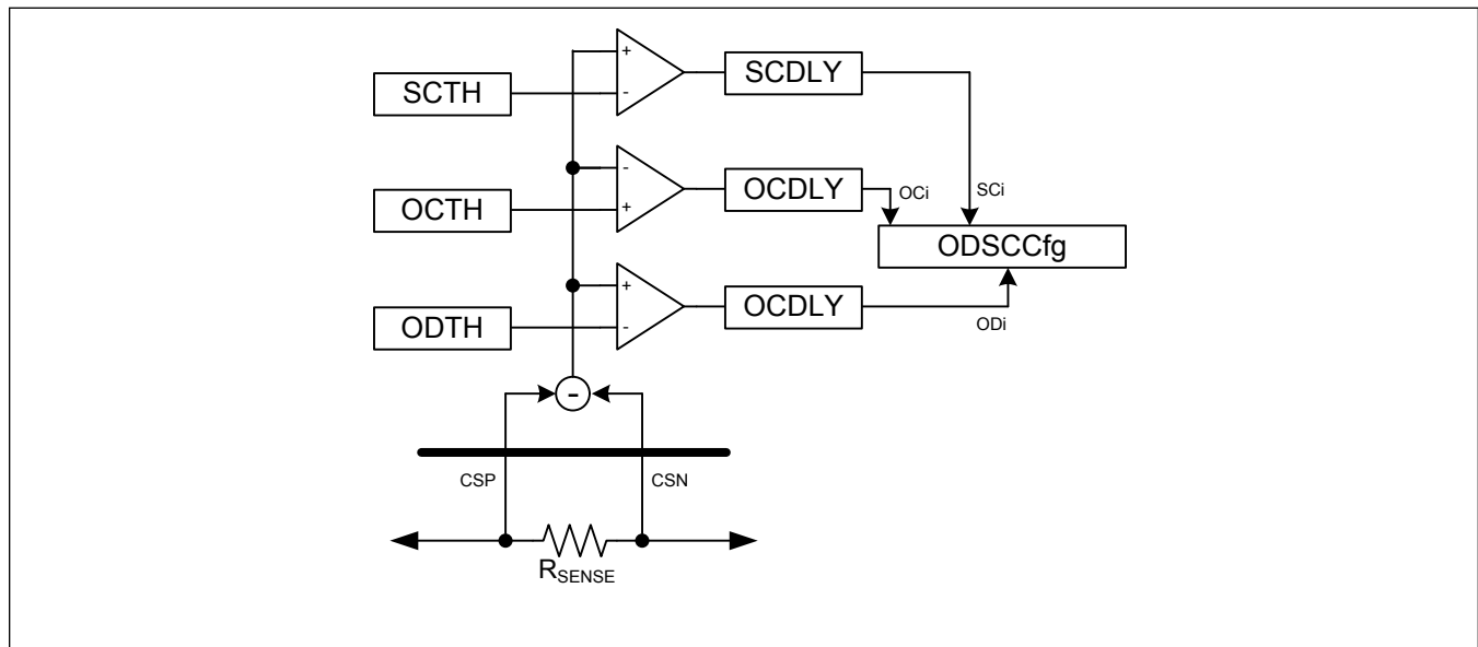
Figure 11. Overcurrent Comparator Diagram
