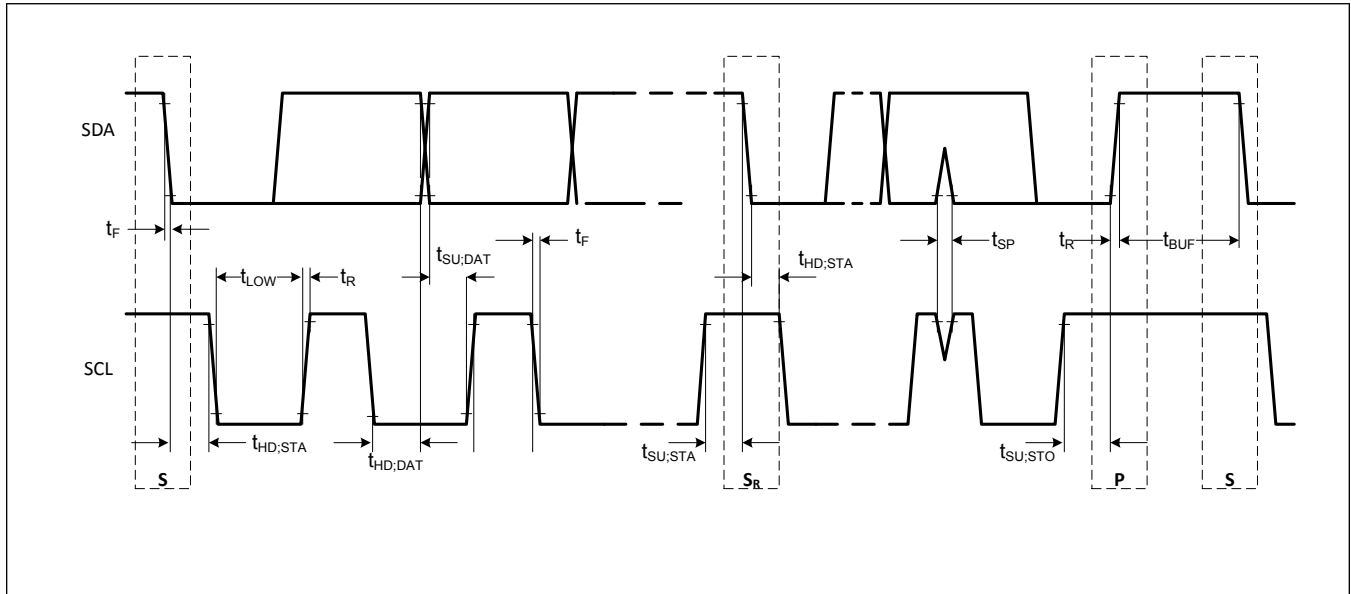
Figure 33. 2-Wire Bus Timing Diagram
