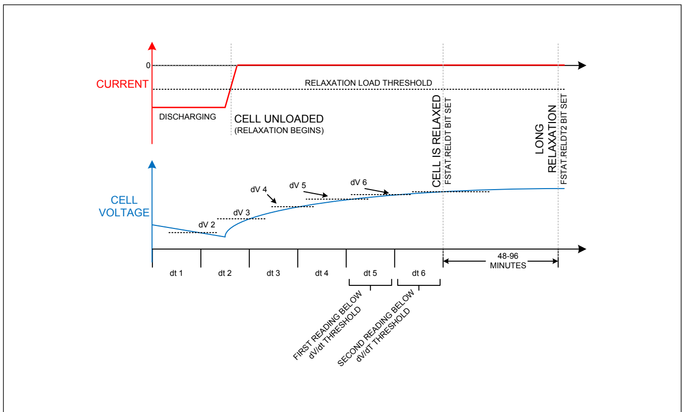
Figure 24. Cell Relaxation Detection
