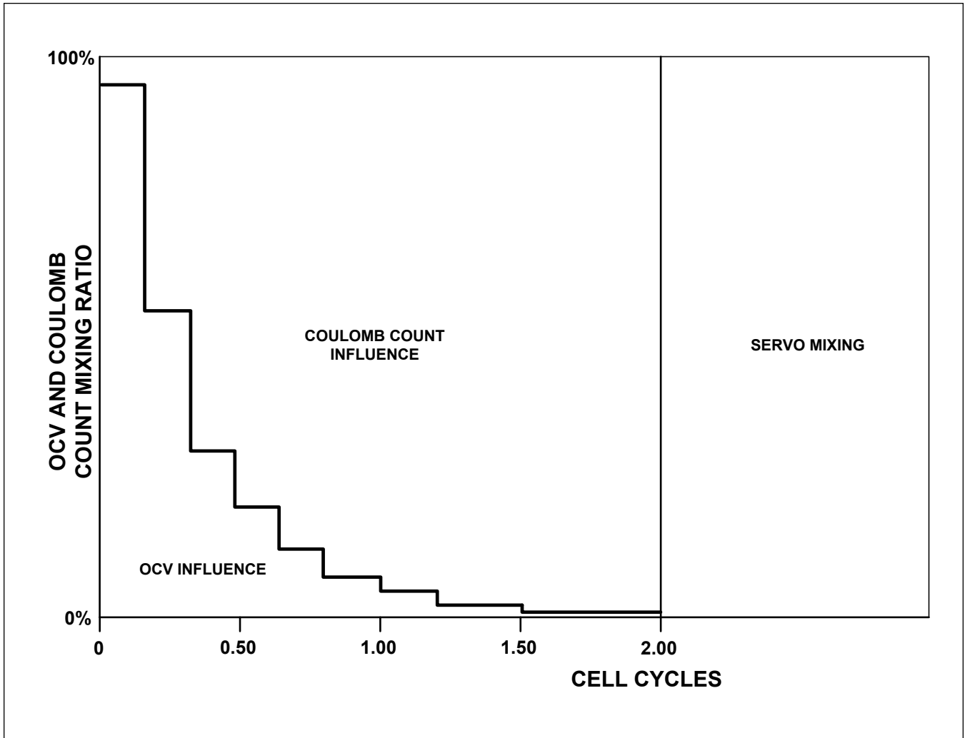
Figure 16. Voltage and Coulomb Count Mixing
