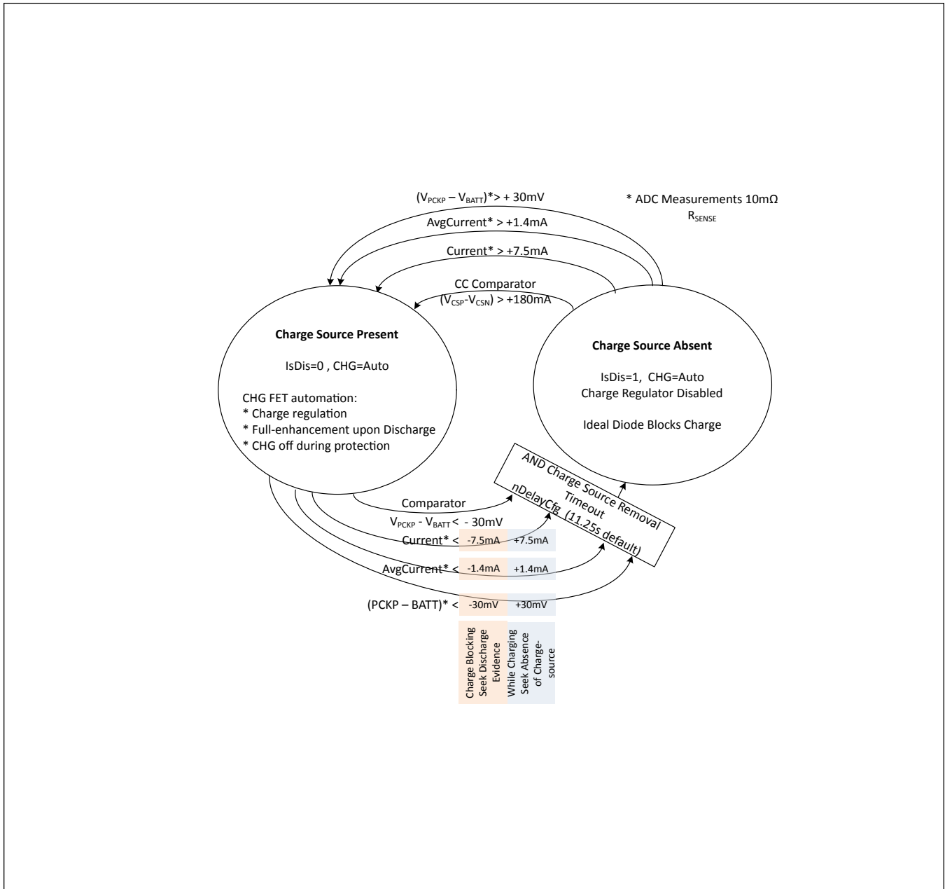
Figure 5. Charging and Discharging States
