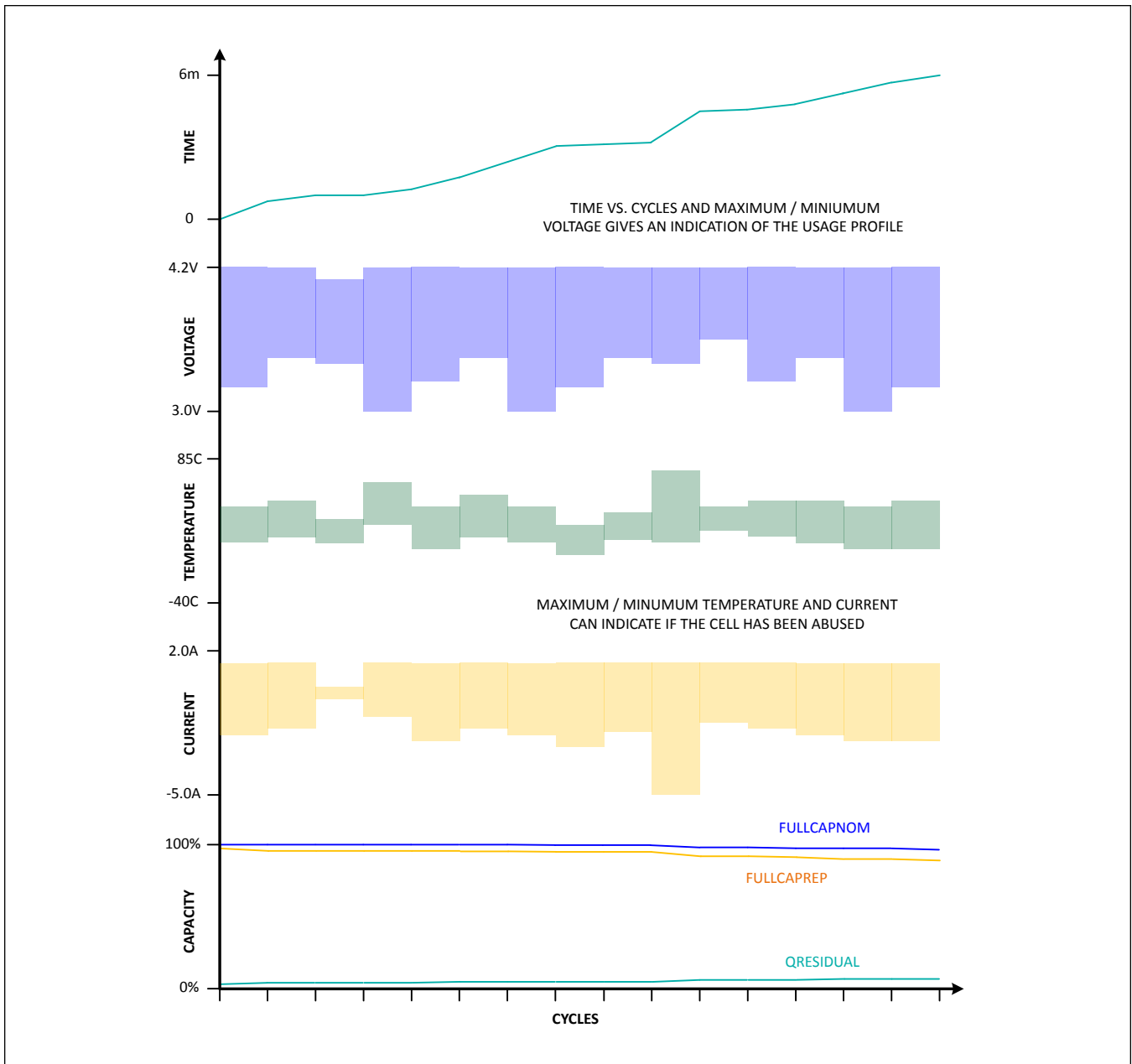
Figure 22. Sample Life Logging Data
