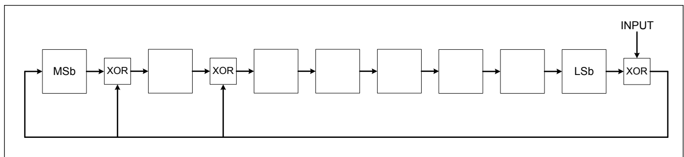
Figure 39. PEC CRC Generation Block Diagram
