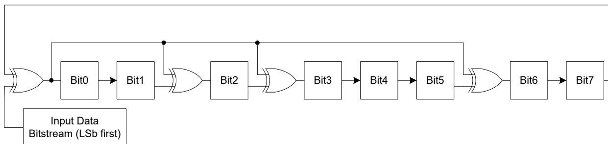
Figure 68. CRC Calculation
