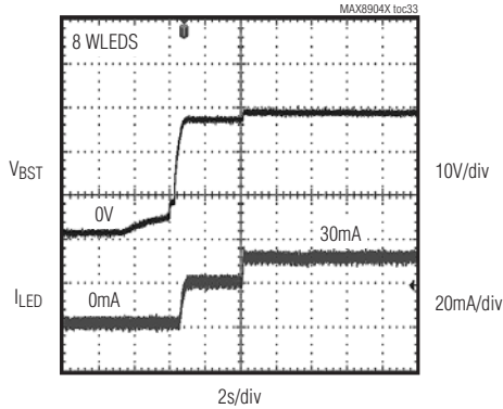
BST STARTUP RESPONSE (CURRENT MODE)
