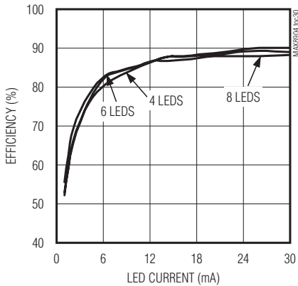
EFFICIENCY vs. LED CURRENT (BST)
