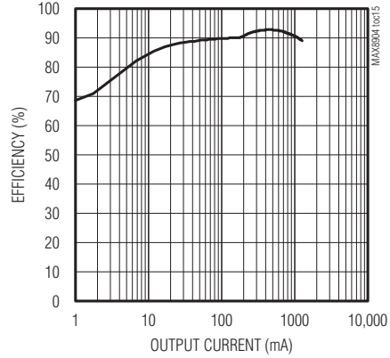
EFFICIENCY vs. OUTPUT CURRENT (3V3)
