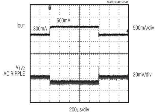
1V2 LOAD TRANSIENT RESPONSE (300mA TO 600mA)
