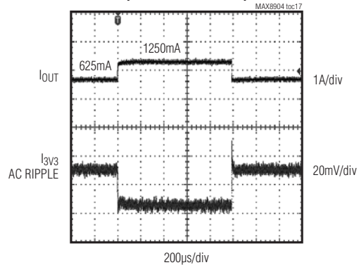
3V3 LOAD TRANSIENT RESPONSE (625mA TO 1250mA)
