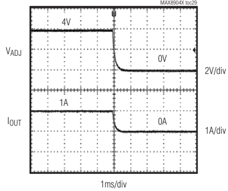
ADJ SHUTDOWN RESPONSE
