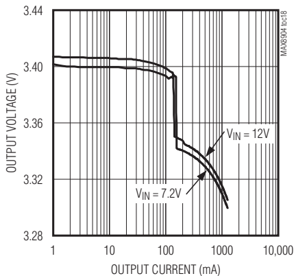
OUTPUT VOLTAGE LOAD REGULATION (3V3)
