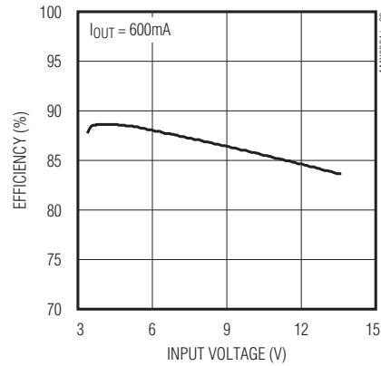
EFFICIENCY vs. INPUT VOLTAGE (1V8)
