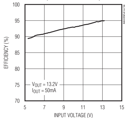
EFFICIENCY vs. INPUT VOLTAGE (BST VOLTAGE MODE)
