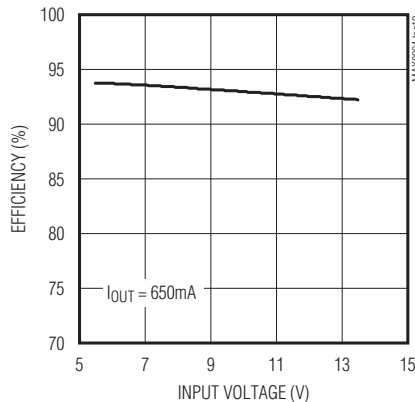
EFFICIENCY vs. INPUT VOLTAGE (5V0)
