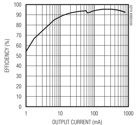
EFFICIENCY vs. OUTPUT CURRENT (5V0)
