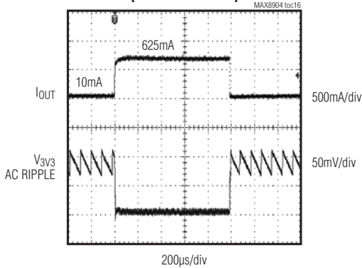
3V3 LOAD TRANSIENT RESPONSE (10mA TO 625mA)
