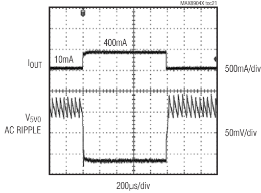
5V0 LOAD TRANSIENT RESPONSE (10mA TO 400mA)
