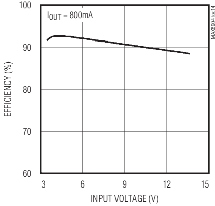
EFFICIENCY vs. INPUT VOLTAGE (3V3)
