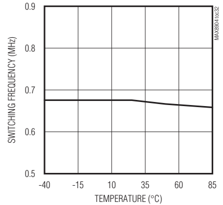
BST SWITCHING FREQUENCY vs. TEMPERATURE
