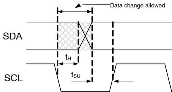
Figure 37. Data Transfer Timing
