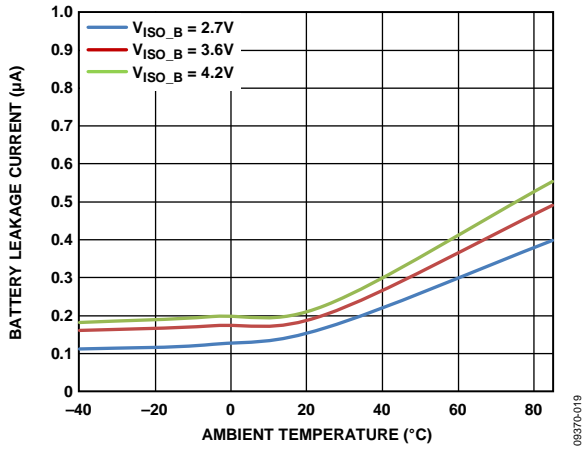
Figure 19. Battery Leakage Current vs. Ambient Temperature
