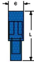
MNU14-156DFI 16-14 Suggested Mate MVU14-156DM
