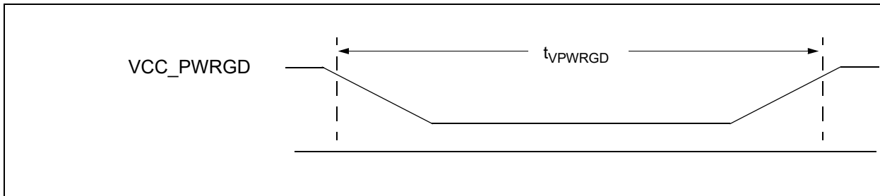
FIGURE 56-4: VCC_PWRGD TIMING
