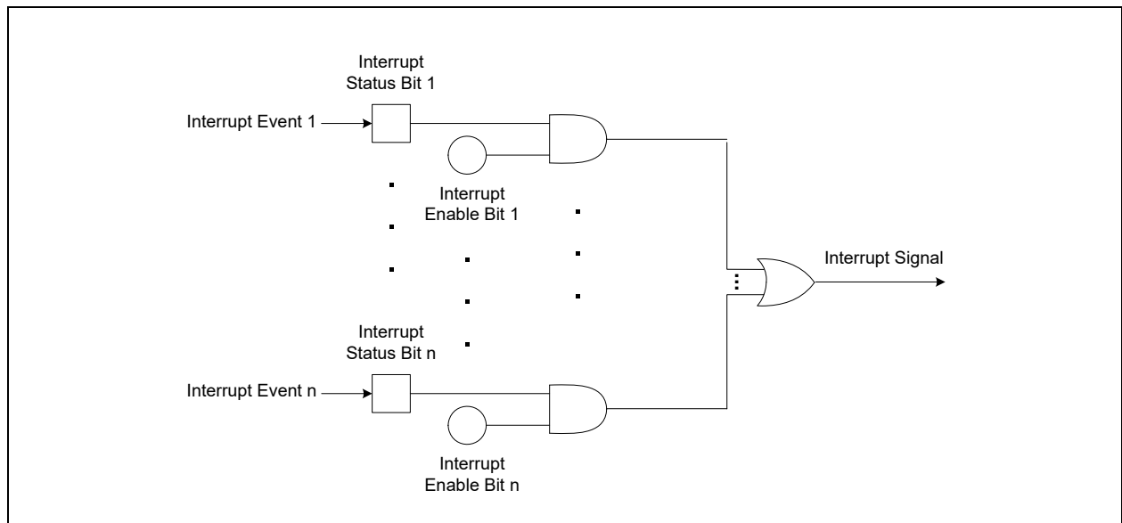
FIGURE 36-4: INTERRUPT FLOW
