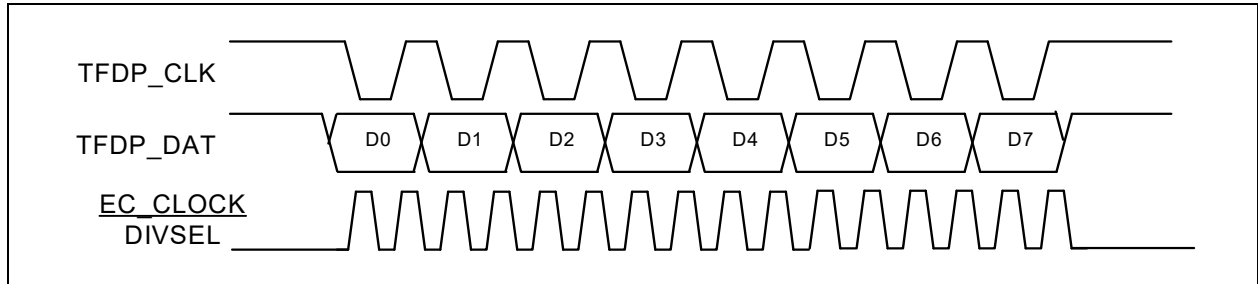
FIGURE 44-3: DATA TRANSFER
