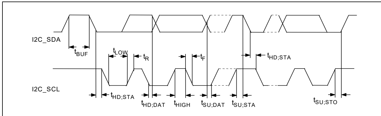
FIGURE 56-15: I2C/SMBUS TIMING
