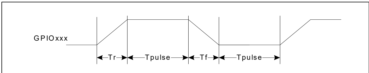
FIGURE 56-7: GPIO TIMING
