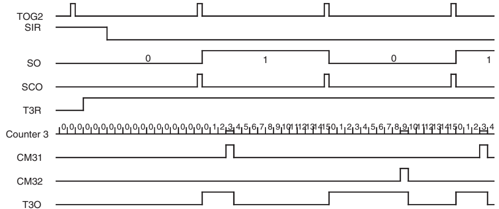
Figure 23-9. Pulse-width Modulation
