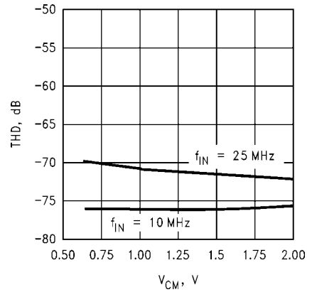
THD vs. V_{CM}
