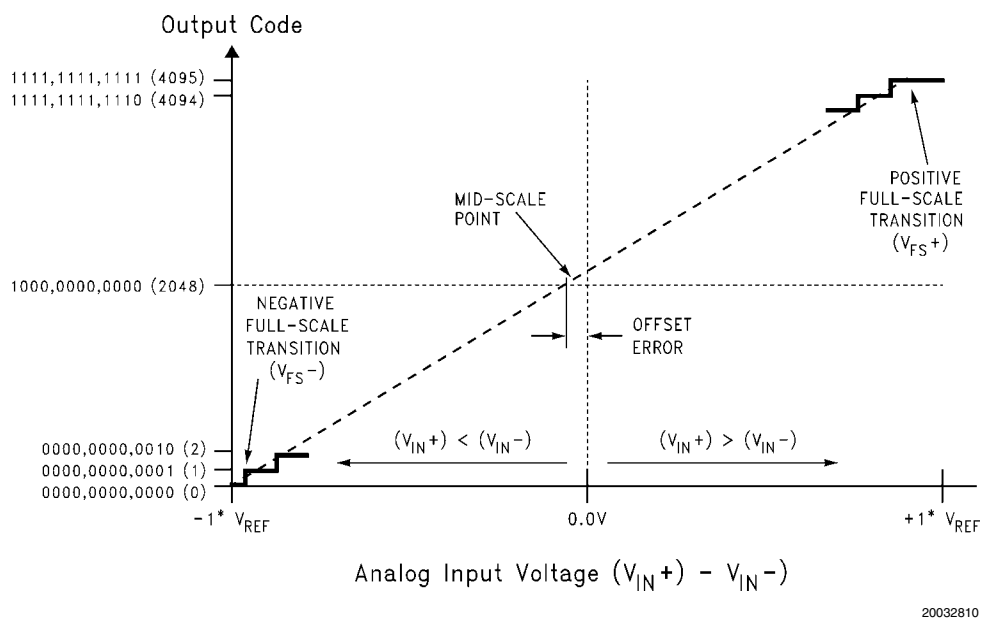
FIGURE 1. Transfer Characteristic
