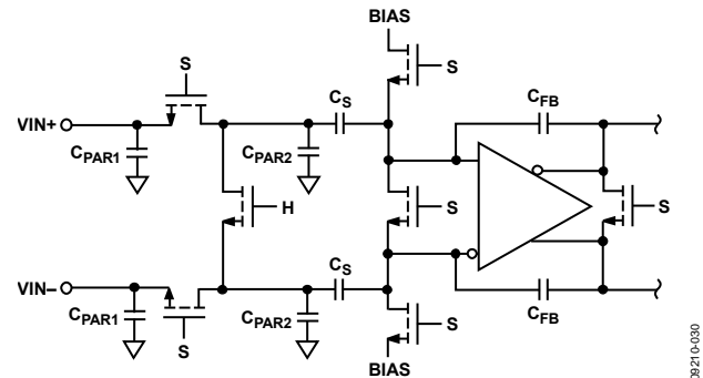
Figure 48. Switched-Capacitor Input
