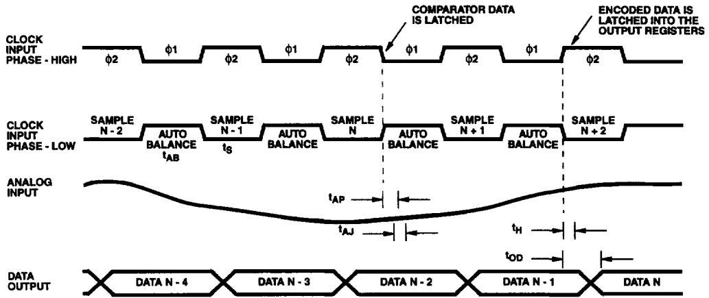
FIGURE 1. INPUT-TO-OUTPUT TIMING
