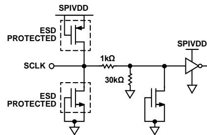
Figure 58. SCLK Input
