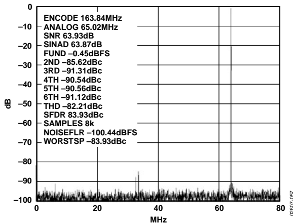
Figure 56. FFT—Using VF561 Crystal as Clock Source
