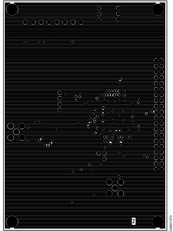
Figure 72. PCB Ground Layer—LVDS
