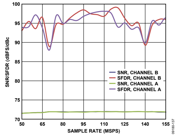
Figure 37. AD9644-155 Single-Tone SNR/SFDR vs. Sample Rate ( f_s ) with f_{IN} = 70. MHz
