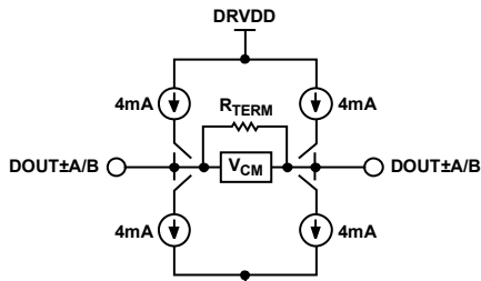
Figure 43. Digital CML Output
