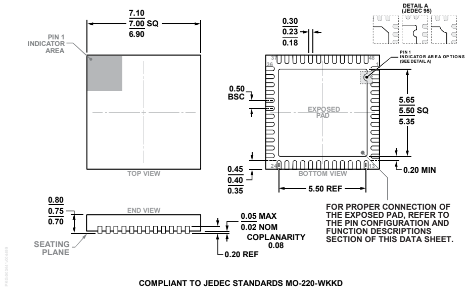
Figure 72. 48-Lead Lead Frame Chip Scale Package [LFCSP] 7 mm × 7 mm Body and 0.75 mm Package Height (CP-48-9) Dimensions shown in millimeters
