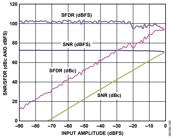
Figure 30. AD9644-155 Single-Tone SNR/SFDR vs. Input Amplitude ( A_{IN} ) with f_{IN} = 180 MHz, f_S = 80 MSPS
