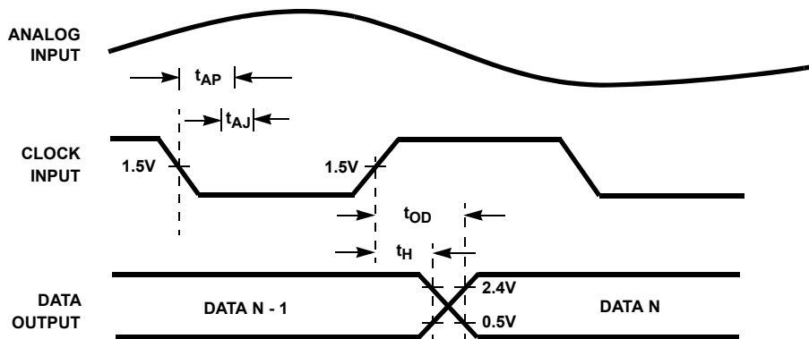
FIGURE 1. HI5766 INTERNAL CIRCUIT TIMING
