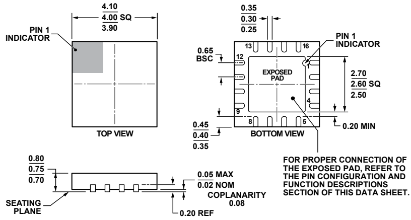
Figure 63. 16-Lead Lead Frame Chip Scale Package [LFCSF_WQ] 4 mm x 4 mm Body, Very Very Thin Quad (CP-16-17) Dimensions shown in millimeters
