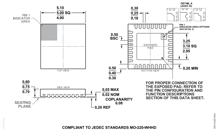
Figure 128. 32-Lead Lead Frame Chip Scale Package [LFCSP] 5 mm × 5 mm Body and 0.75 mm Package Height (CP-32-7) Dimensions shown in millimeters
