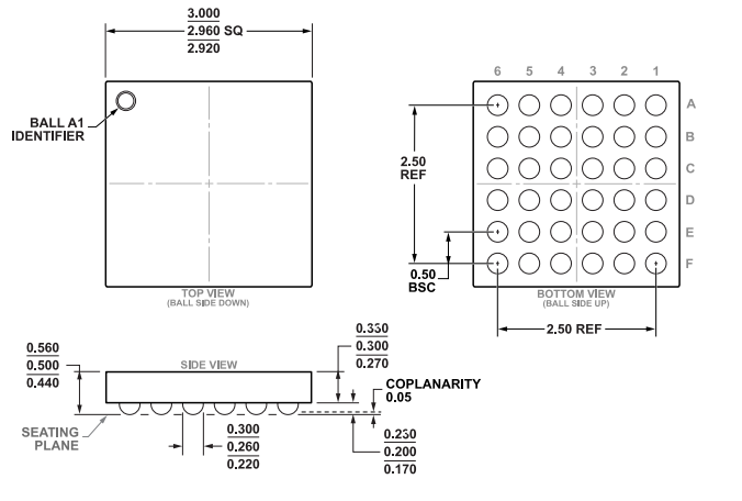
Figure 129. 36-Ball Wafer Level Chip Scale Package (WL CSP) (CB-36-5) Dimensions shown in millimeters
