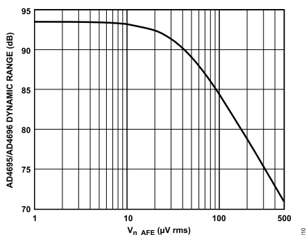
Figure 114. AD4695/AD4696 Typical Dynamic Range vs. v_{n\_AFE} , V_{REF} = 5 \text{ V}
