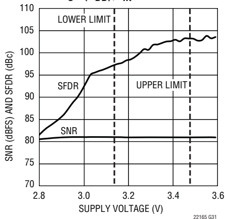
LTC2216 SNR and SFDR vs Supply Voltage ( V_{DD} ), f_{IN} = 5.1\text{MHz}
