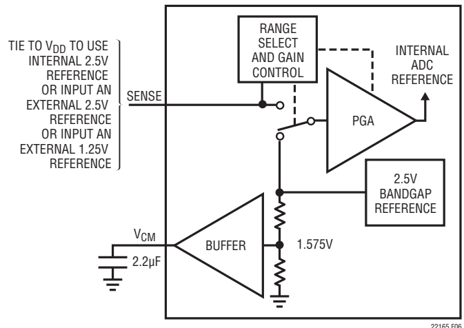
Figure 6. Reference Circuit
