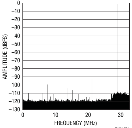
LTC2215 64k Point FFT, f_{IN} = 28.7\text{MHz} , -1\text{dBFS}
