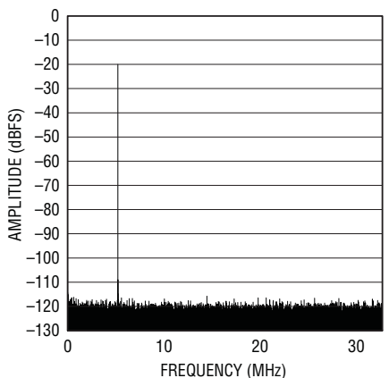
LTC2215 64k Point FFT, f_{IN} = 70.1\text{MHz} , -20\text{dBFS} , Dither "On"
