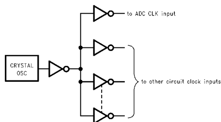
FIGURE 7. Clock Tree for Clock Isolation
