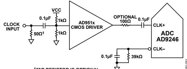
150Ω RESISTOR IS OPTIONAL Figure 49. Single-Ended 1.8 V CMOS Sample Clock
