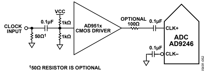
150Ω RESISTOR IS OPTIONAL Figure 50. Single-Ended 3.3 V CMOS Sample Clock
