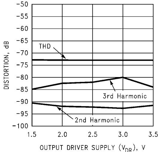
Distortion vs. V_{DR} @ f_{IN} = 4.7 MHz
