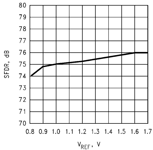
SFDR vs. V_{REF} @ f_{IN} = 4.7 MHz
