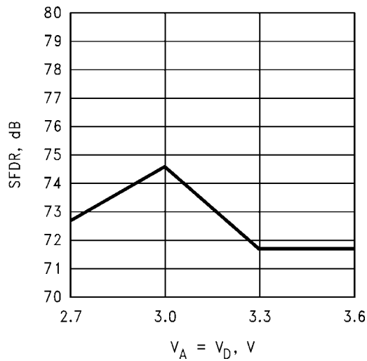
SFDR vs. Supply Voltage @ f_{IN} = 4.7 MHz
