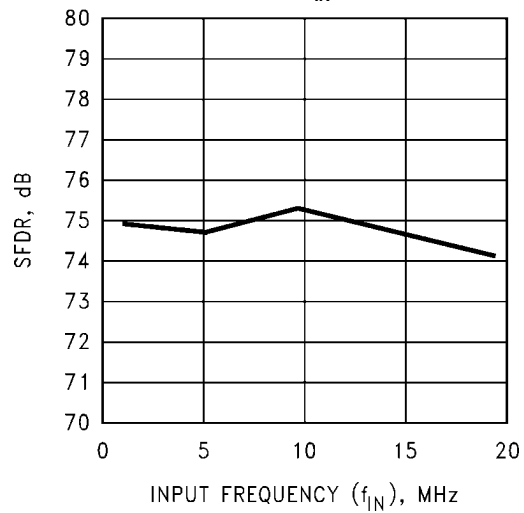
SFDR vs. f_{IN}
