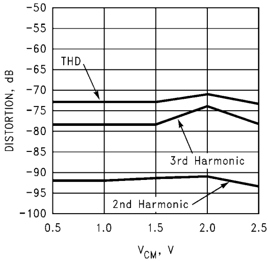
Distortion vs. V_{CM} @ f_{IN} = 4.7 MHz
