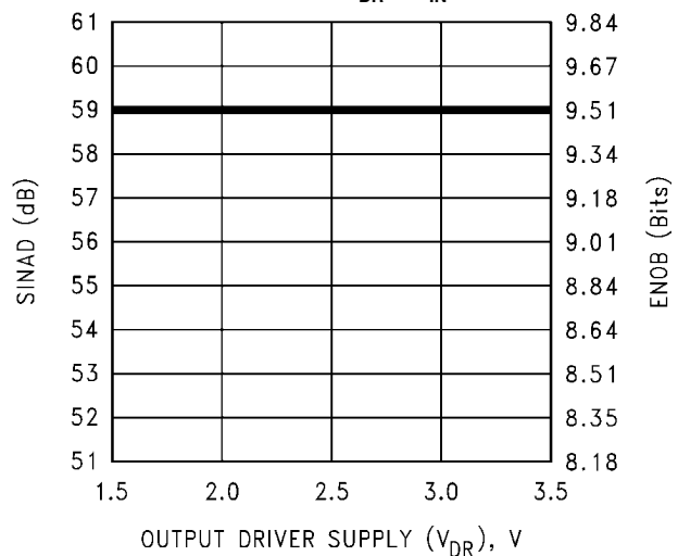
SINAD & ENOB vs. V_{DR} @ f_{IN} = 9.5 MHz
