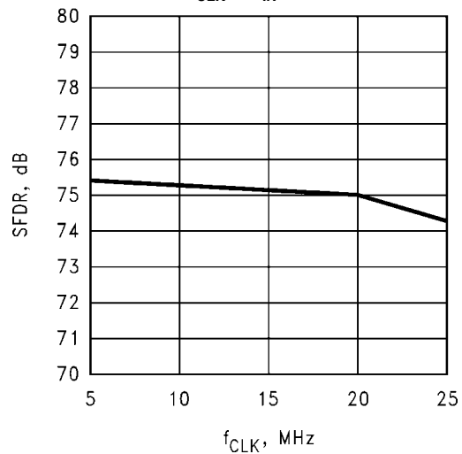
SFDR vs. f_{CLK} @ f_{IN} = 9.5 MHz
