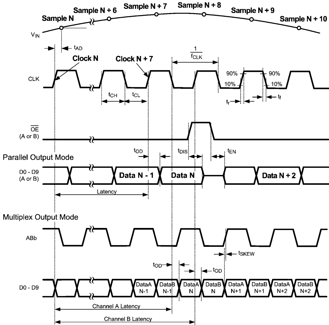
Output Timing
