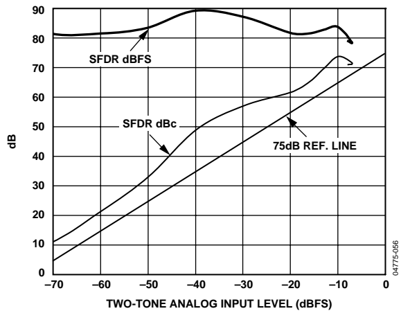
Figure 21. Two-Tone IMD Performance vs. Input Drive Level (69.1 MHz and 70.1 MHz; f_s = 65 MSPS (-65 Grade); F_1, F_2 Levels Equal)
