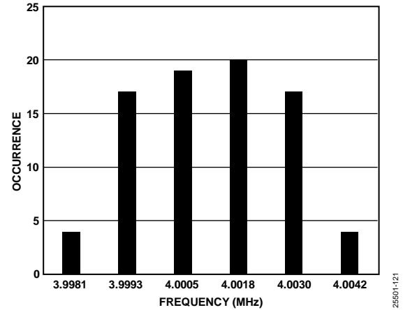
Figure 21. Internal Oscillator Frequency and Accuracy Distribution Histogram
