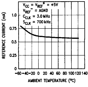
Reference Current (I REF ) vs Ambient Temperature
