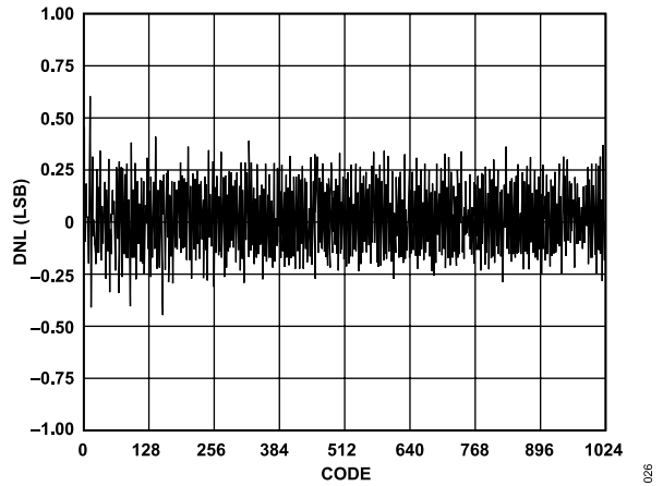
Figure 21. DNL @ 80 MSPS
