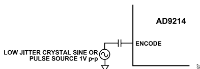
Figure 27. AC-Coupled Encode Circuit
