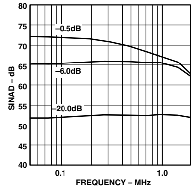
TPC 6. SINAD vs. Input Frequency (Input Span = 5.0 V p-p, V_{\text{CM}} = 2.5 \text{ V} )
