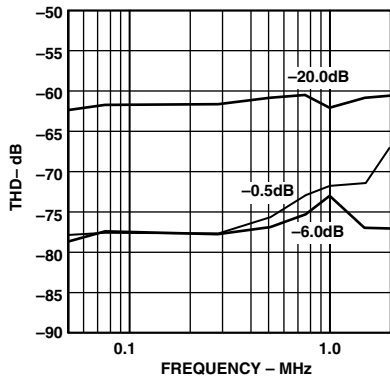
TPC 7. THD vs. Input Frequency (Input Span = 5.0 V p-p, V_{\text{CM}} = 2.5 \text{ V} )
