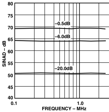
TPC 4. SINAD vs. Input Frequency (Input Span = 2.0 V p-p, V_{\text{CM}} = 2.5 \text{ V} )
