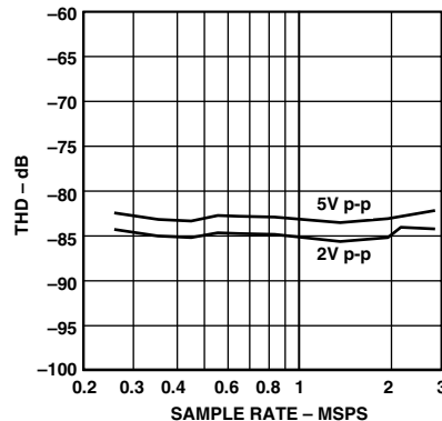
TPC 8. THD vs. Sample Rate ( A_{\text{IN}} = -0.5 \text{ dB} , f_{\text{IN}} = 500 \text{ kHz} , V_{\text{CM}} = 2.5 \text{ V} )
