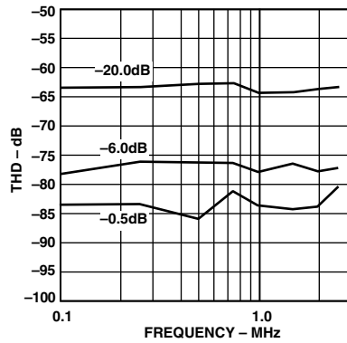
TPC 5. THD vs. Input Frequency (Input Span = 2.0 V p-p, V_{\text{CM}} = 2.5 \text{ V} )
