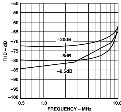
TPC 23. THD vs. Input Frequency (Input Span = 2.0 V p-p, V_{\text{CM}} = 2.5 \text{ V} )
