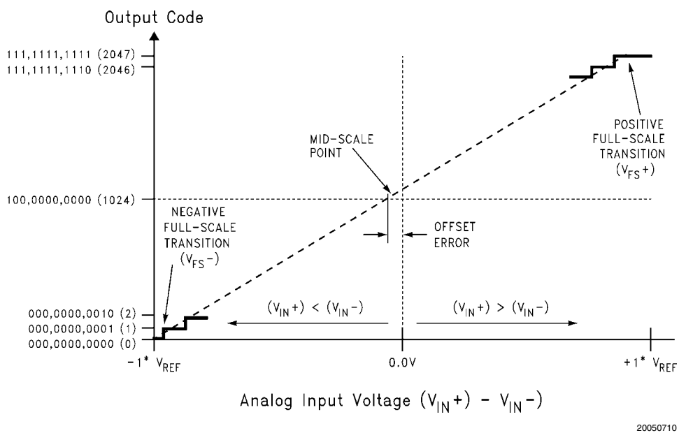
FIGURE 1. Transfer Characteristic
