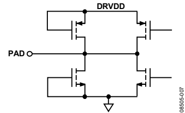
Figure 57. Digital Output
