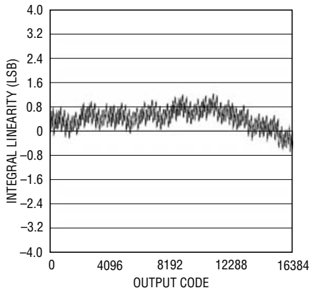
Integral Linearity End Point Fit for CHO with Internal 2.5V Reference, Unipolar Mode
