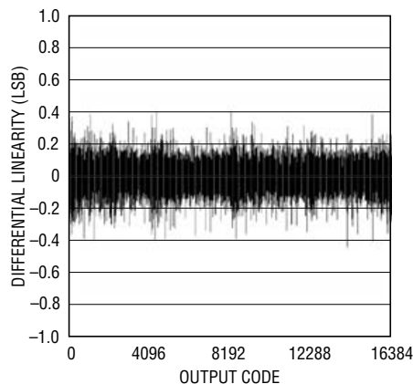
Differential Linearity for CHO with Internal 2.5V Reference, Differential Input in Bipolar Mode
