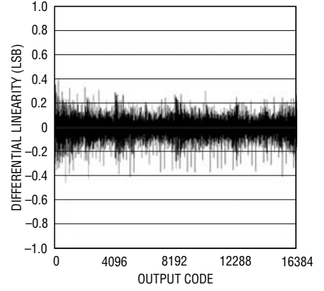
Differential Linearity for CHO with Internal 2.5V Reference, Unipolar Mode
