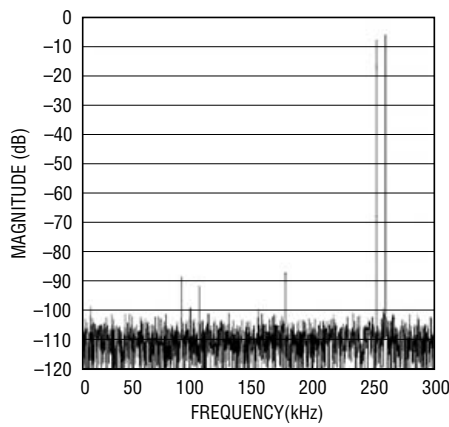
833kHz into CHO +, 841kHz into CHO -, 588ksps Bipolar Mode 4096 Point FFT
