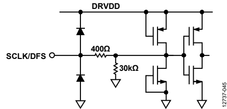
Figure 41. Equivalent SCLK/DFS Input Circuit
