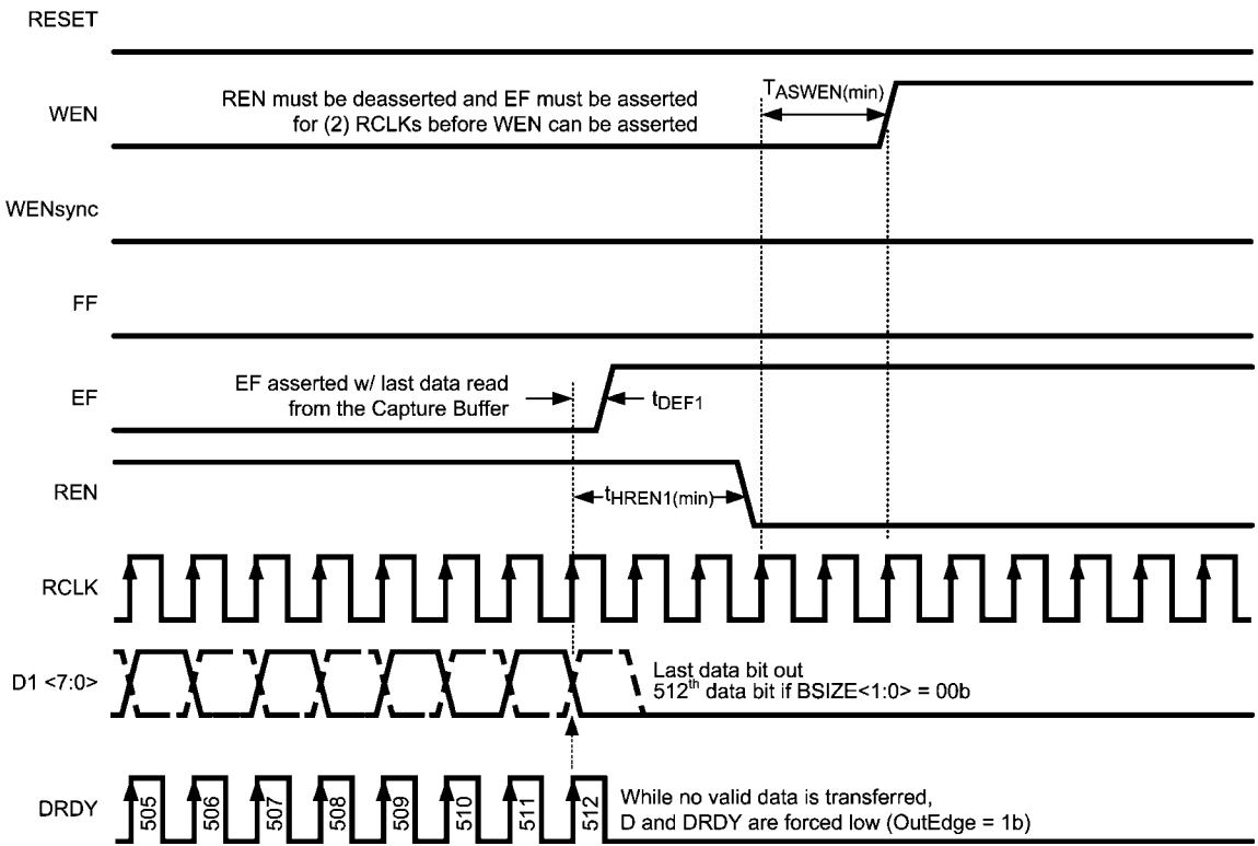
FIGURE 10. Capture Buffer End of READ Phase (OutEdge = 1b)(Notes 14, 15)
