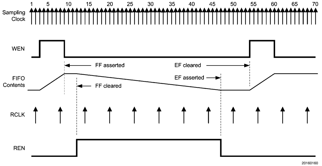
FIGURE 5. Capture Buffer Read Operation
