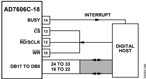
Figure 98. AD7606C-18 Interface Diagram—One AD7606C-18 Using the Parallel Bus with \overline{CS} and \overline{RD} Shorted Together
