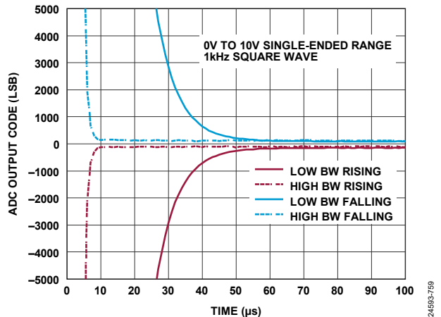
Figure 68. Step Response, 0 V to 10 V Single-Ended Range, Fine Settling
