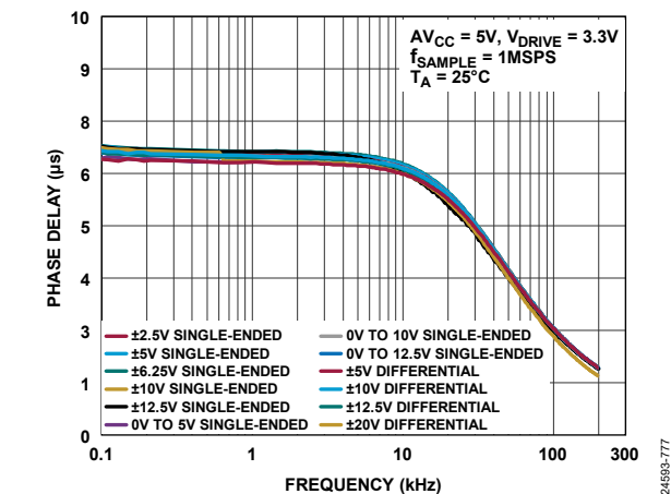
Figure 78. Analog Antialiasing Filter Phase Response, Low Bandwidth Mode
