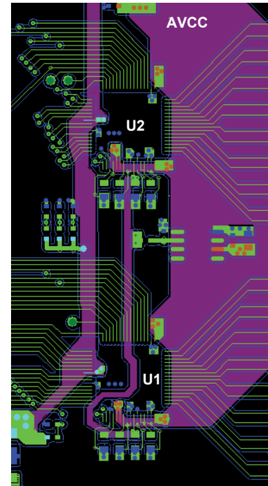
Figure 124. Layout for Multiple AD7606C-18 Devices—Top Layer and Supply Plane Layer
