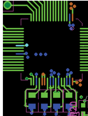
Figure 122. Top Layer Decoupling REFIN/REFOUT, REFCAPA, REFCAPB, and REGCAP Pins
