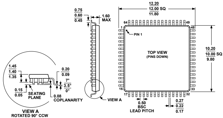
Figure 126. 64-Lead Low Profile Quad Flat Package [LQFP] (ST-64-2) Dimensions shown in millimeters
