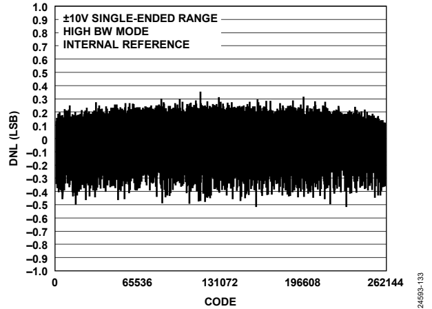
Figure 42. Typical DNL, High Bandwidth Mode
