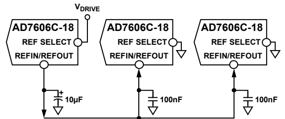
Figure 85. Internal Reference Driving Multiple AD7606C-18 REF IN /REF OUT Pins
