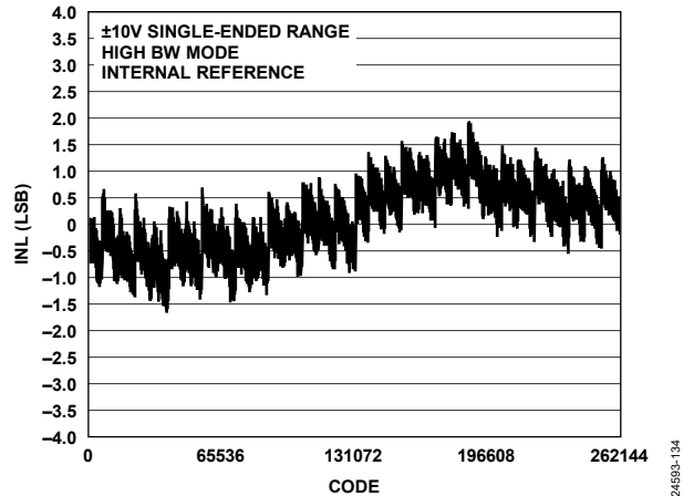
Figure 43. Typical INL, High Bandwidth Mode
