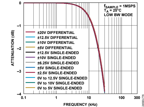
Figure 77. Analog Antialiasing Filter Frequency Response, Low Bandwidth Mode
