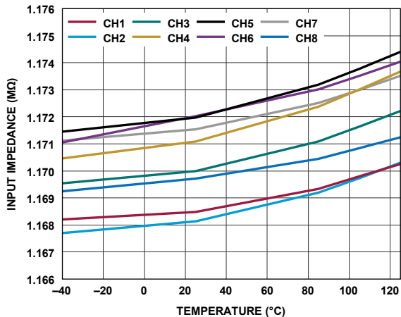
Figure 71. Input Impedance vs. Temperature
