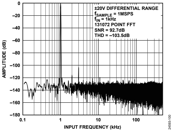
Figure 9. Fast Fourier Transform (FFT), ±20 V Differential Range, Low Bandwidth Mode
