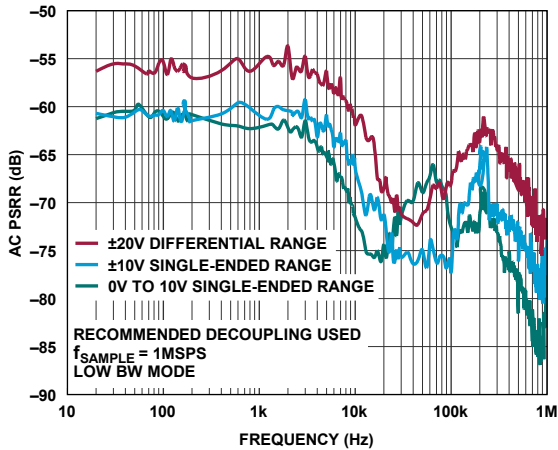
Figure 70. AC Power Supply Rejection Ratio (PSRR) vs. Frequency, Low Bandwidth Mode
