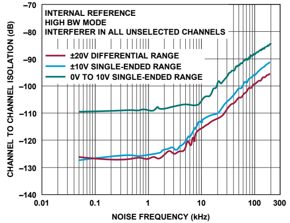
Figure 72. Channel to Channel Isolation vs. Noise Frequency, High Bandwidth Mode
