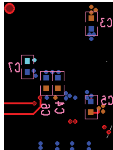
Figure 123. Bottom Layer Decoupling
