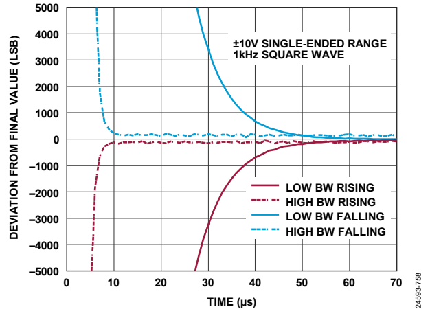
Figure 67. Step Response, \pm 10 V Single-Ended Range, Fine Settling
