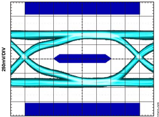
0.125UI/DIV AT 2.25Gbps Figure 5. Rx Eye Diagram at TP2 (Cable = 2 m, 30 AWG)
