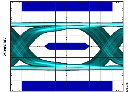
0.125UI/DIV AT 2.25Gbps Figure 7. Rx Eye Diagram at TP3 (Cable = 2 m, 30 AWG)
