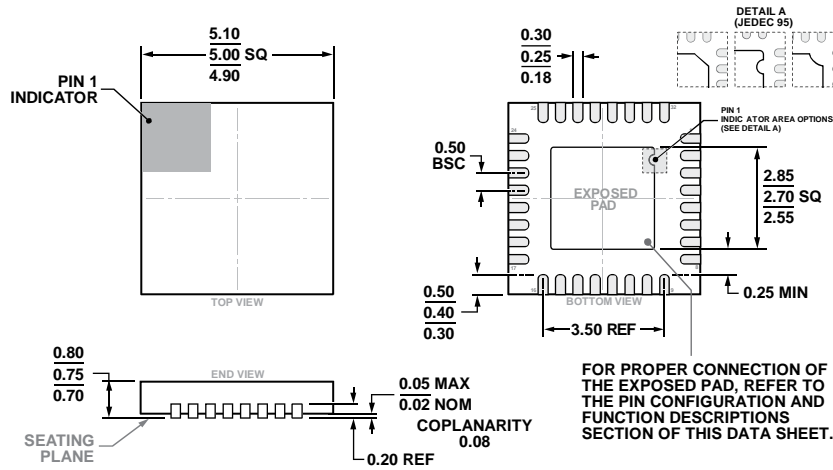
Figure 27. 32-Lead Lead Frame Chip Scale Package [LFCSP] 5 mm × 5 mm Body and 0.75 mm Package Height (CP-32-21)
