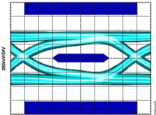
0.125UI/DIV AT 2.25Gbps Figure 6. Rx Eye Diagram at TP2 (Cable = 6 m, 24 AWG)
