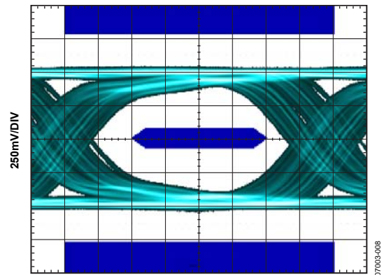
0.125UI/DIV AT 2.25Gbps Figure 8. Rx Eye Diagram at TP3 (Cable = 6 m, 24 AWG)
