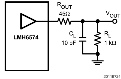
FIGURE 6. Decoupling Capacitive Loads
