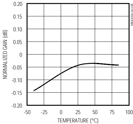
GAIN vs. TEMPERATURE MAX4356 toc108
