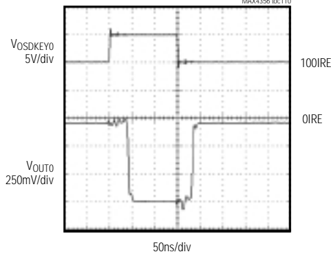
OSD SWITCHING TRANSIENT (100IRE LEVEL SWITCH) MAX4356 toc110
