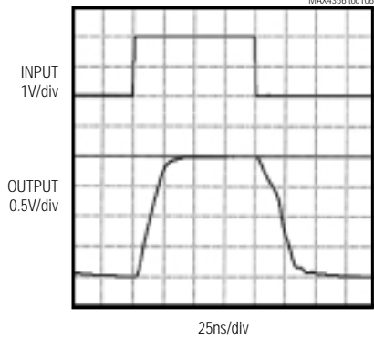
LARGE-SIGNAL PULSE RESPONSE WITH CAPACITIVE LOAD ( C_L = 30pF ) MAX4356 toc106
