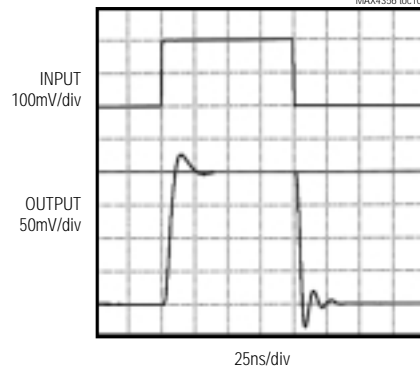
MEDIUM-SIGNAL PULSE RESPONSE WITH CAPACITIVE LOAD ( C_L = 30pF ) MAX4356 toc107
