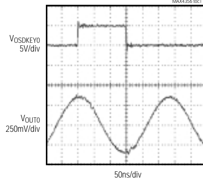
OSD SWITCHING 3.58MHz SIGNAL MAX4356 toc111
