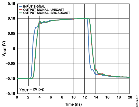
Figure 15. ADV3224 Large Signal Pulse Response
