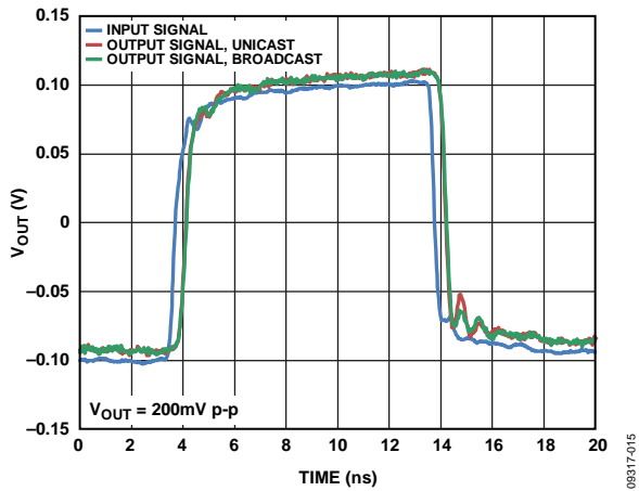
Figure 14. ADV3224 Small Signal Pulse Response
