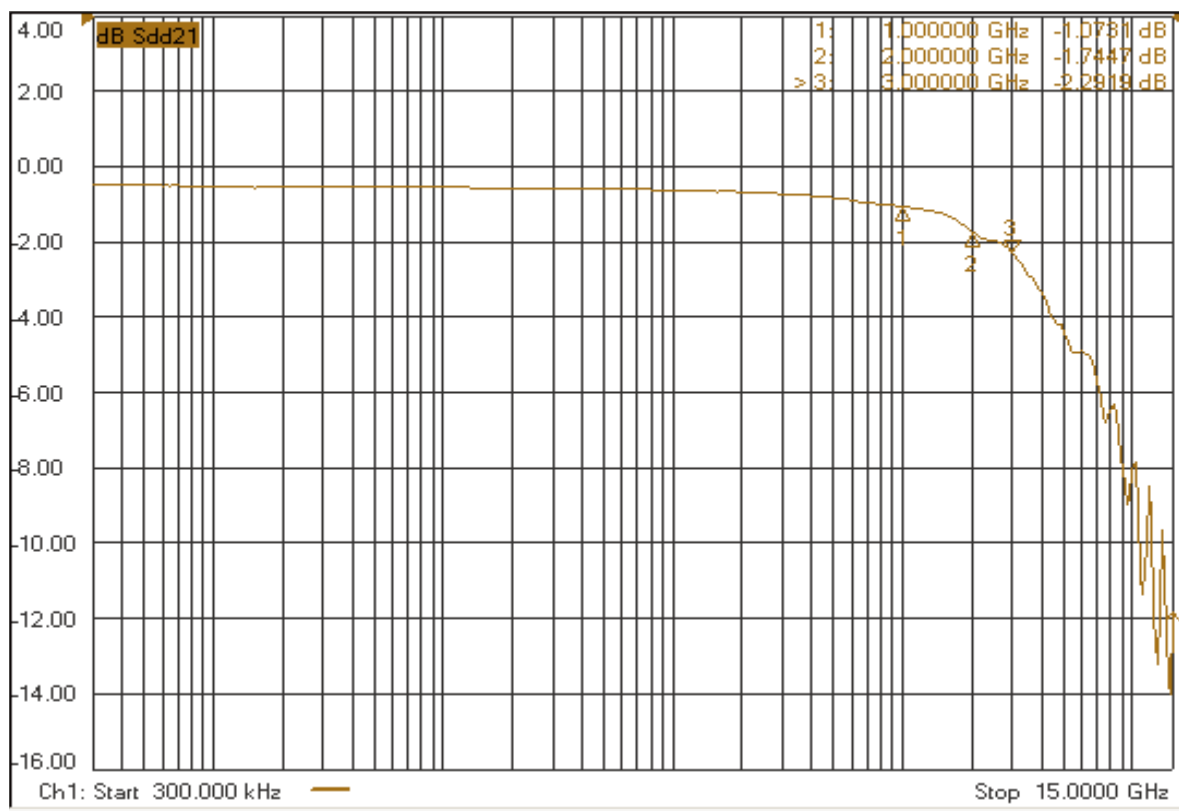
Insertion Loss
