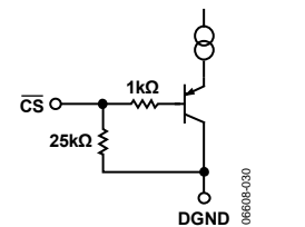
Figure 17. \overline{CS} Input (Also See ESD Protection Map, Figure 19)
