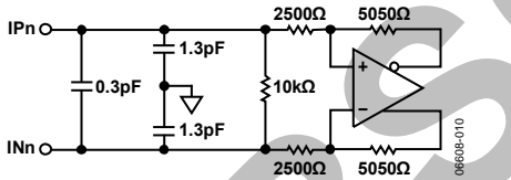
Figure 10. Receiver Differential (Also See ESD Protection Map, Figure 19)
