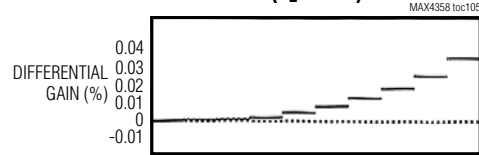
DIFFERENTIAL GAIN AND PHASE ( R_L = 1k\Omega )
